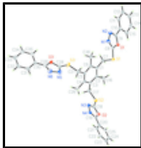
Fig. 1. View of (I) showing the atom-labelling scheme. Displacement ellipsoids are drawn at the 50% probability level.
